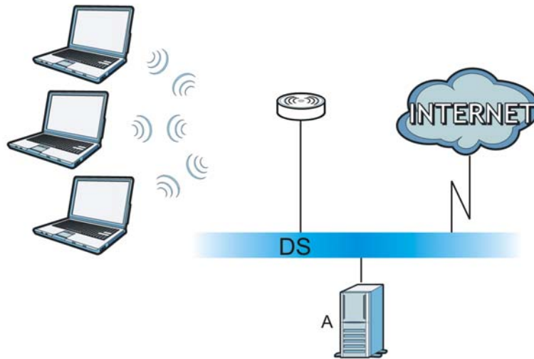
Figure 93 WPA2 with RADIUS Application Example
