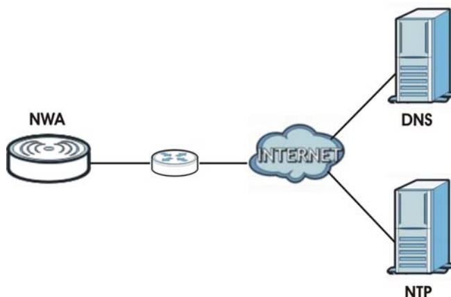
Figure 56 NWA Setup
